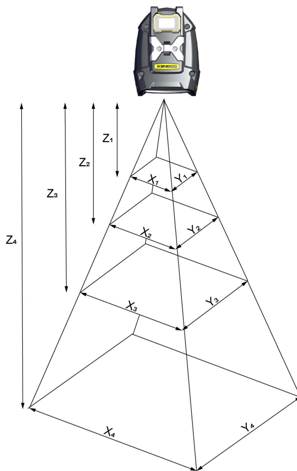
DM8700 LX Field of View Values
