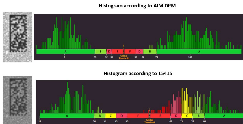
Contrast Calculation Differences – 15415 and AIM-DPM
